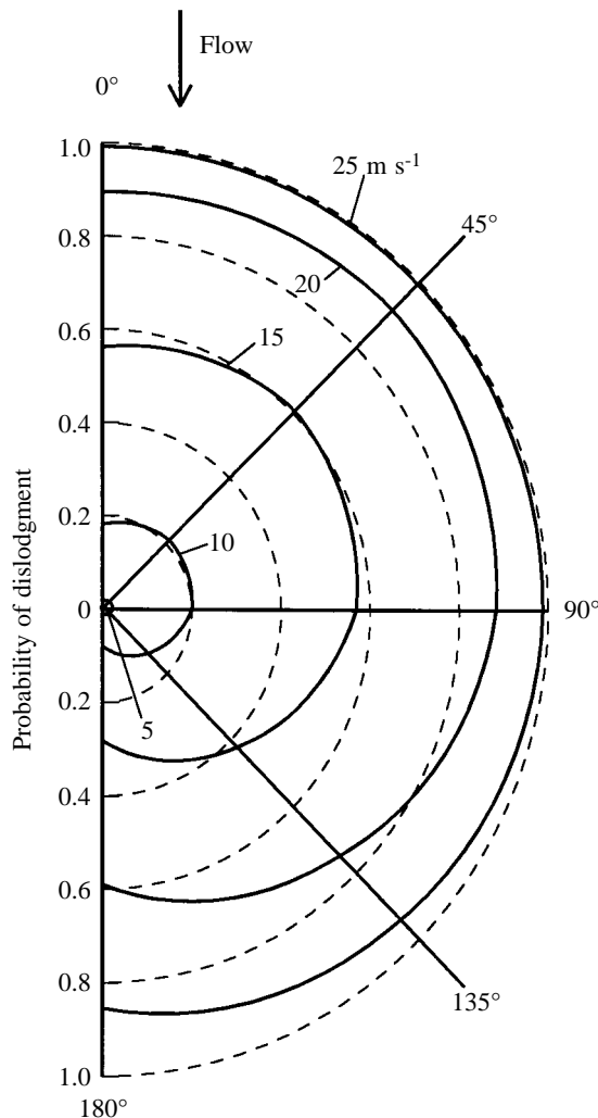
Fig. 12. The probability of dislodgment as a function of orientation to flow and water velocity for a moving limpet. Values are plotted as for Fig. 11.
